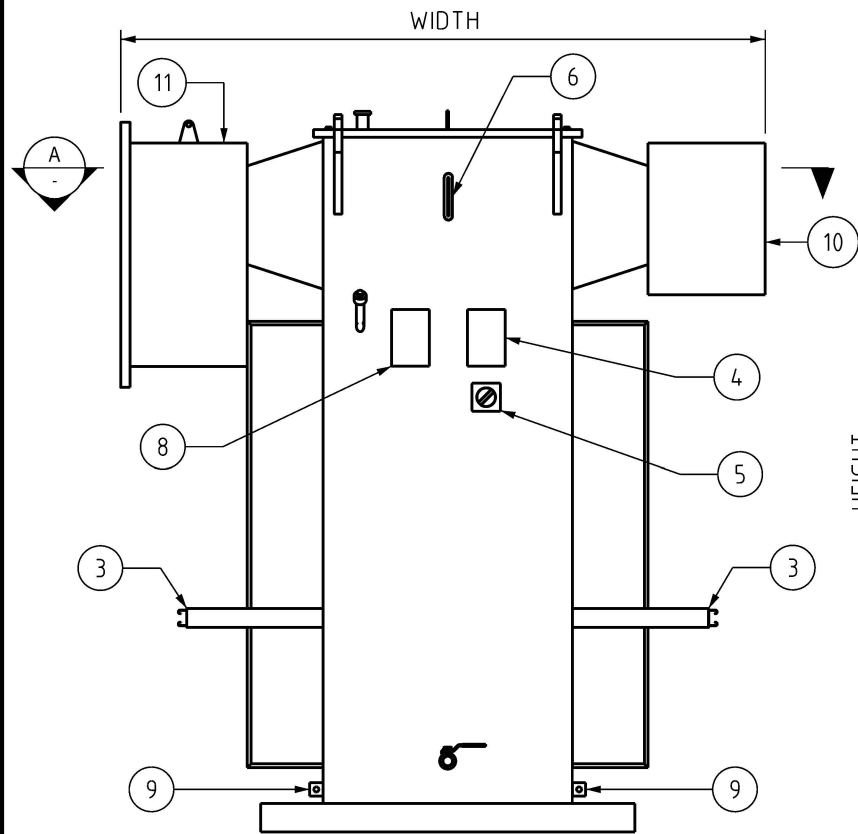
FRONT ELEVATION
