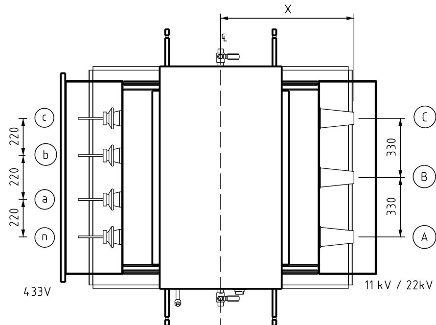
SECTION VIEW
