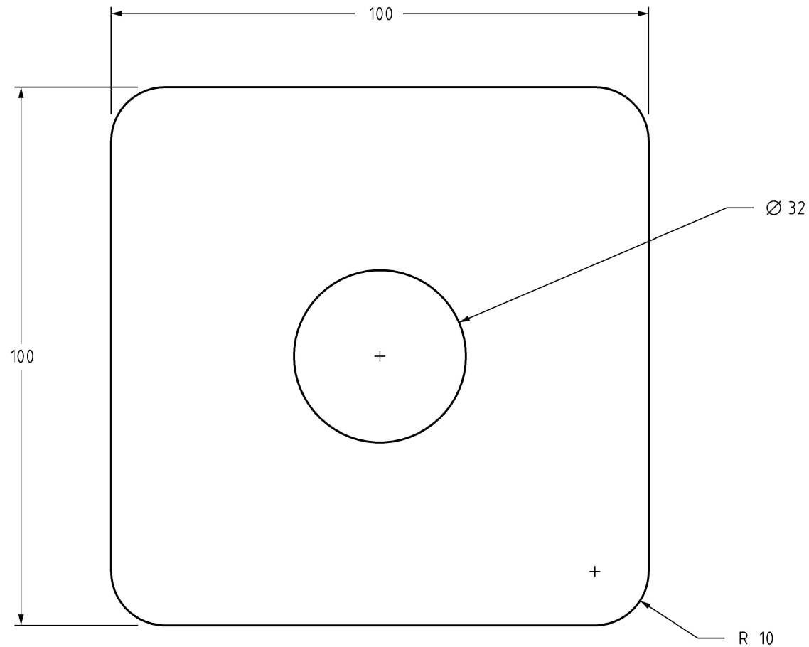
TOP VIEW SCALE 1:1
