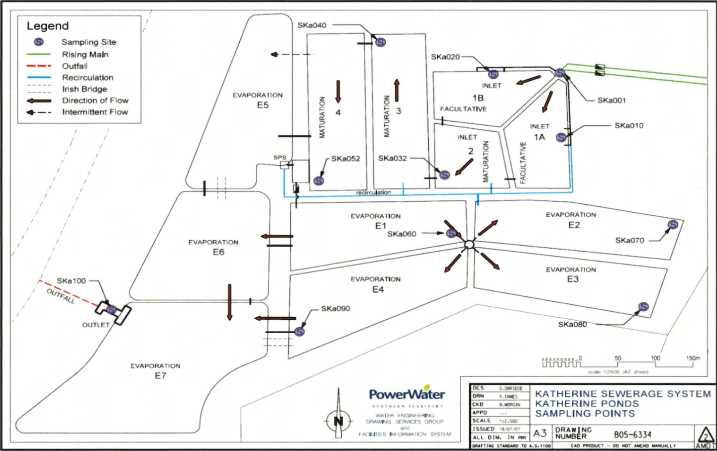
Figure 1 - Site plan and flow diagram for Katherine Wastewater Treatment Plant
