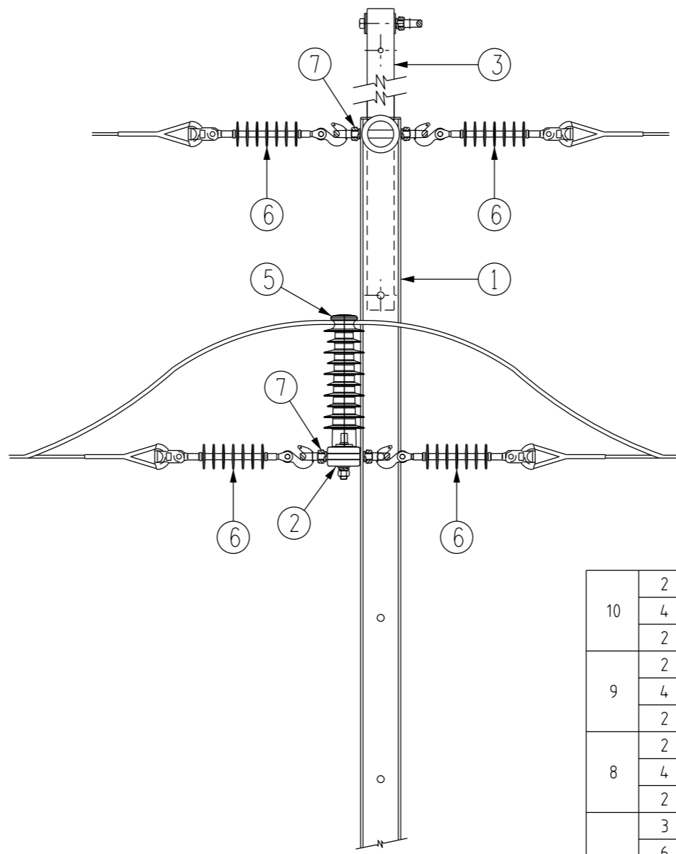
END ELEVATION/SECTION CROSSARM BRACE NOT SHOWN FOR CLARITY
