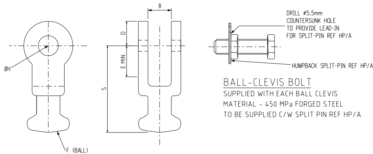
ITEM 4: BALL-CLEVIS TO BE SUPPLIED WITH BOLT MATERIAL - FORGED STEEL
