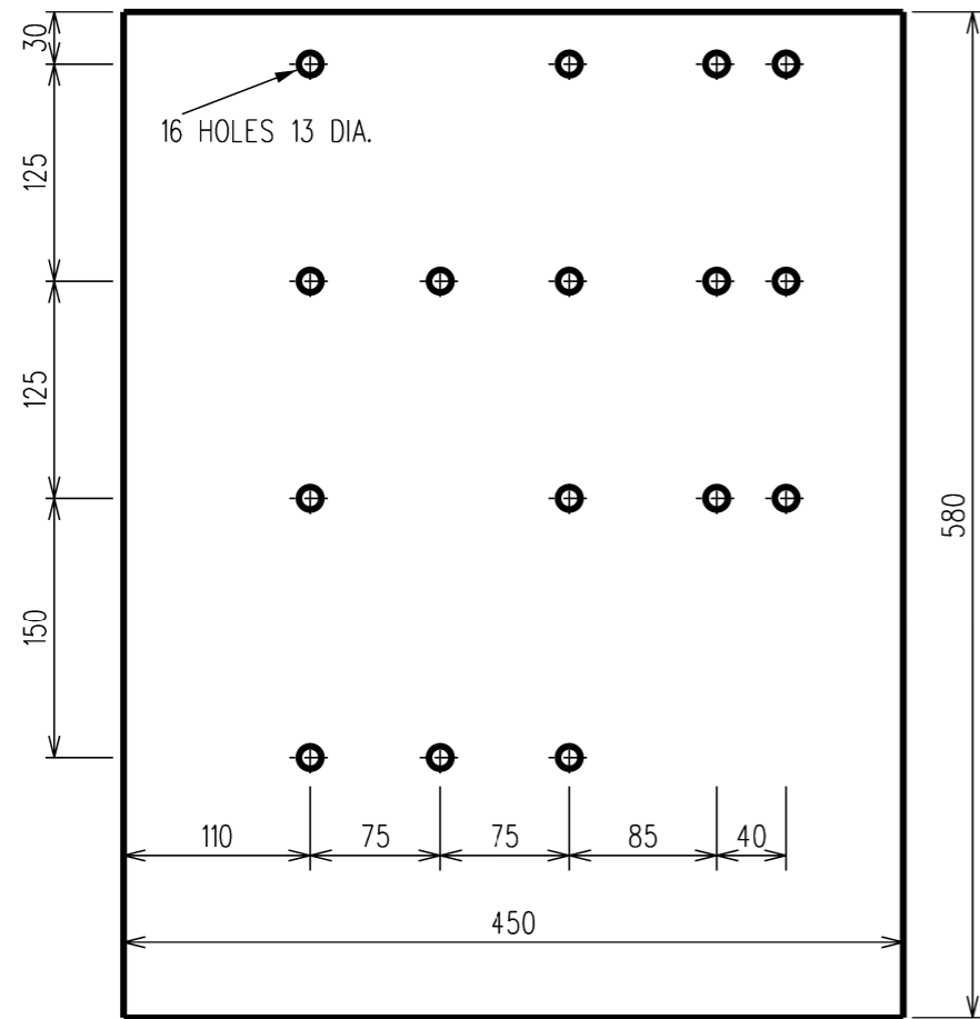
ITEM 1 - INSULATING PANEL
