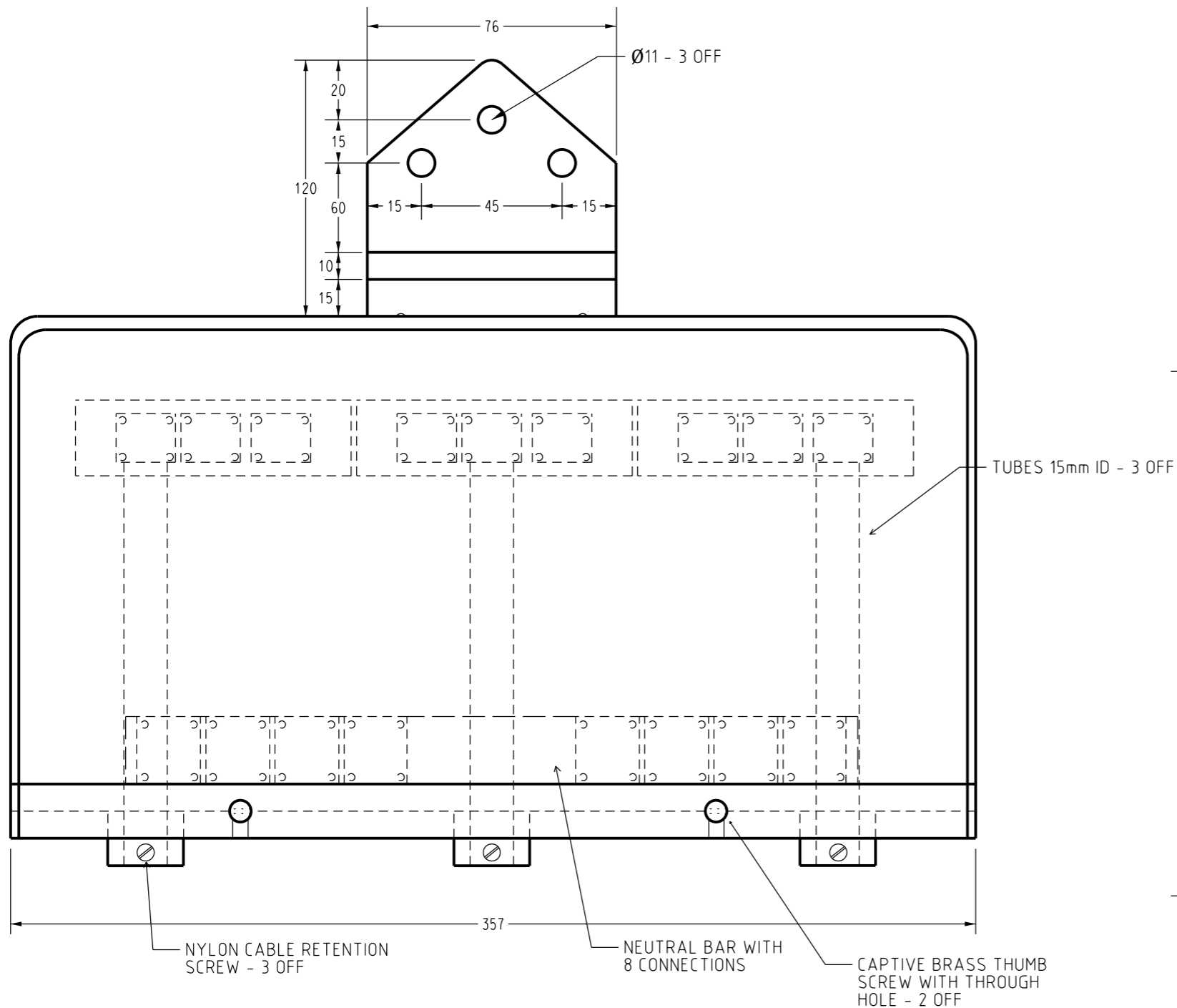
1 FRONT ELEVATION SCALE 1:2
