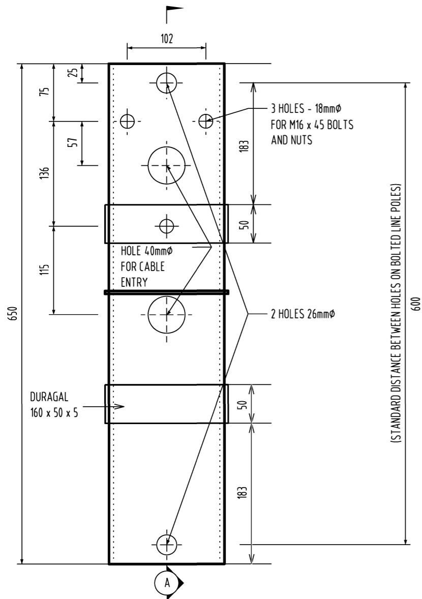
ITEM 1 MOUNTING BRACKET ITEM NUMBER 401396
