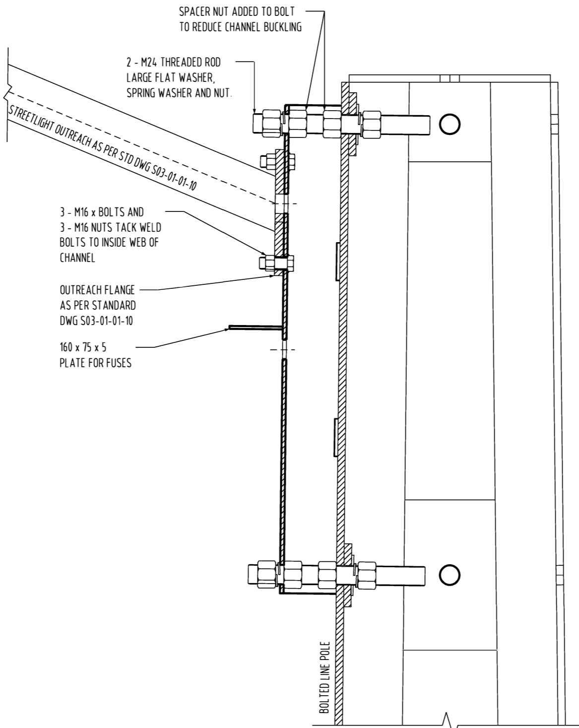
ITEM 1 MOUNTING BRACKET ITEM NUMBER 401396
