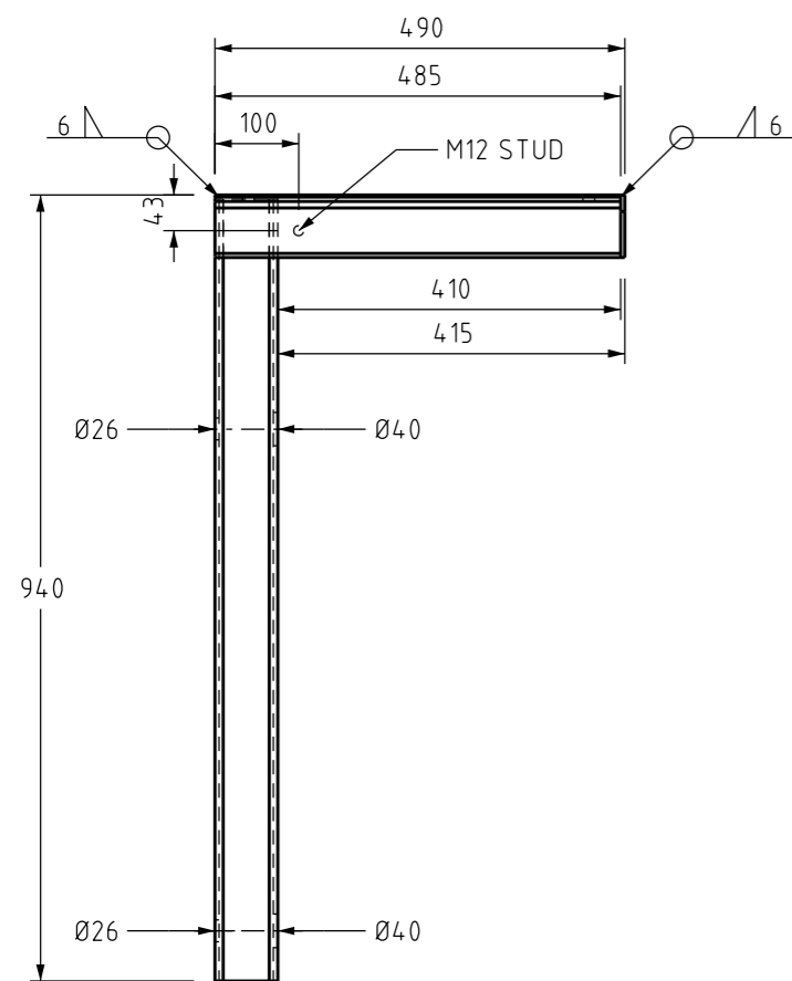
TOP VIEW 1:10
