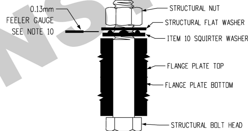
TYPICAL BOLT HOLE ASSEMBLY
