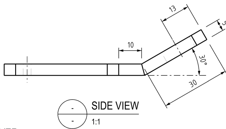
SWITCH COVER 5mm THICK ALUMINIUM PLATE
