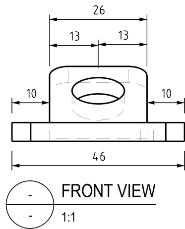
SWITCH COVER 5mm THICK ALUMINIUM PLATE
