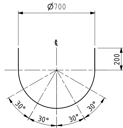
TOP VIEW SCALE ( 1 : 20 )
