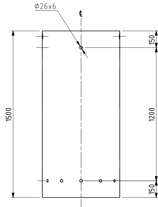
FRONT VIEW SCALE ( 1 : 20 )
