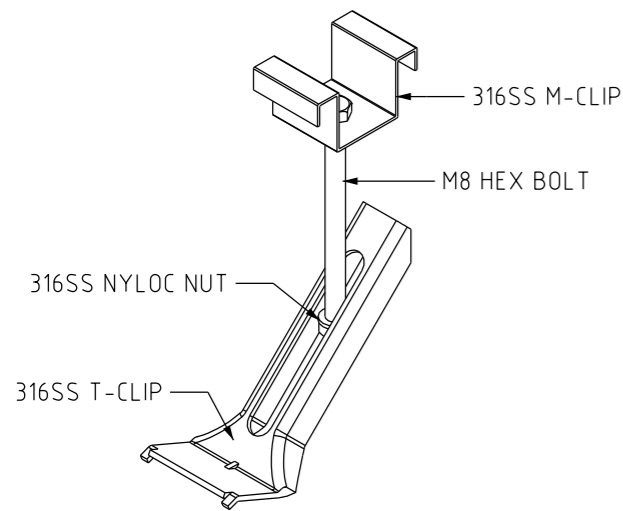
M-T CLIP ASSEMBLY ISOMETRIC VIEW N.T.S.
