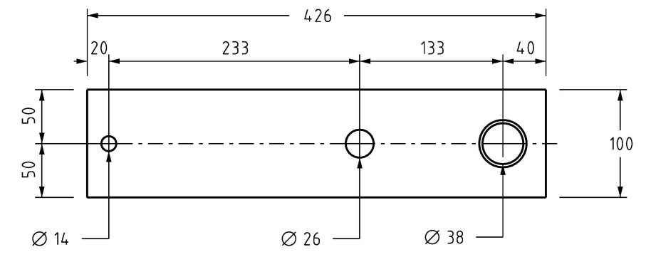
TOP VIEW 1:5
