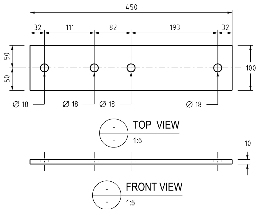
LV 'B' TOP PLATE MATERIAL: 100 x 10 MILD STEEL CF ITEM NUMBER : 298661 HOT DIPPED GALVANIZED ITEM NUMBER : 411556
