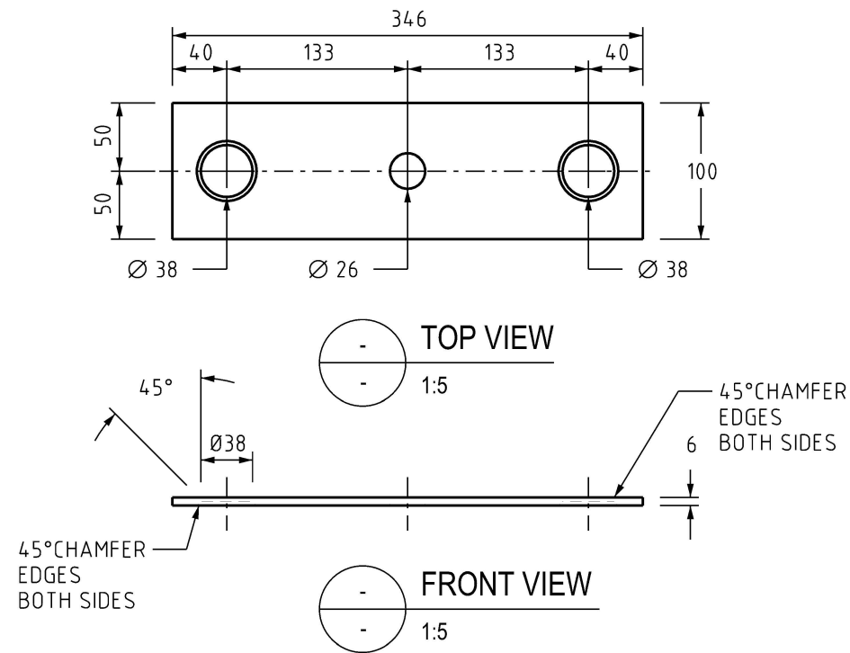
HV STRAIN PLATE (FOR METAL AND 125x125 FIBREGLASS X-ARM) MATERIAL: 100 x 6 DURAGAL CF ITEM NUMBER: 406938
