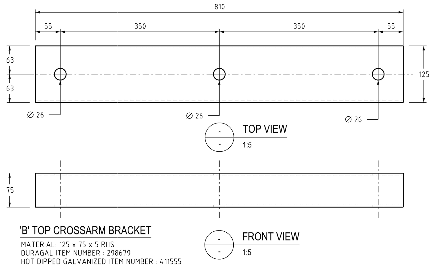
HV STRAIN PLATE (FOR 200x100 FIBREGLASS X-ARM) MATERIAL: 100 x 6 CF DURAGAL ITEM NUMBER : 298653
