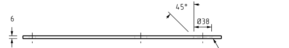
FRONT VIEW 1:5
