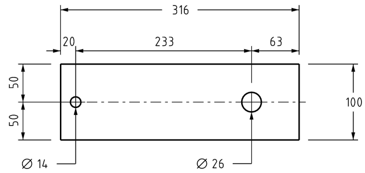
TOP VIEW 1:5
